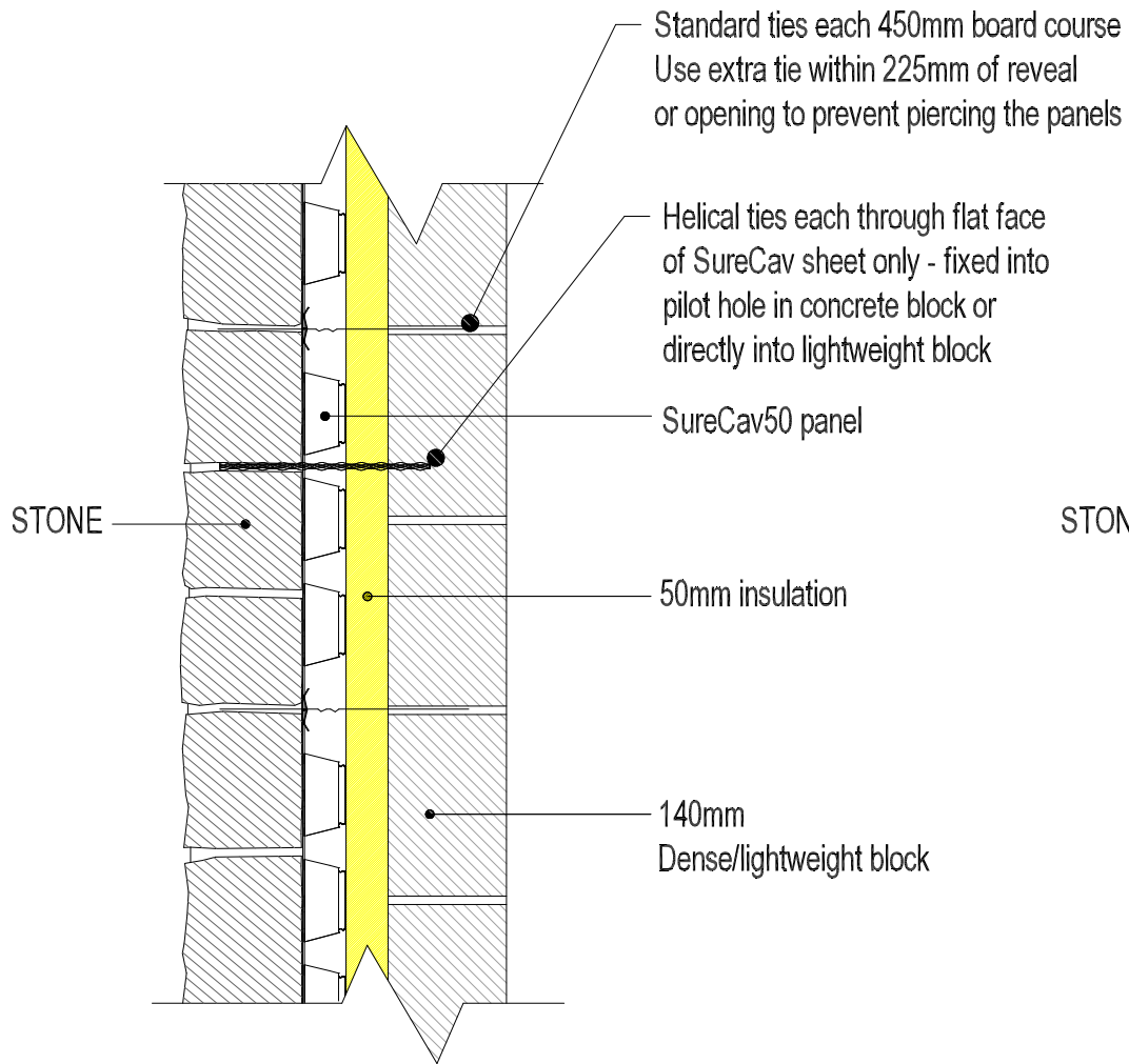
SURECAV50 WALL-TIE OPTION WITH DENSE OR LIGHTWEIGHT BLOCKS
