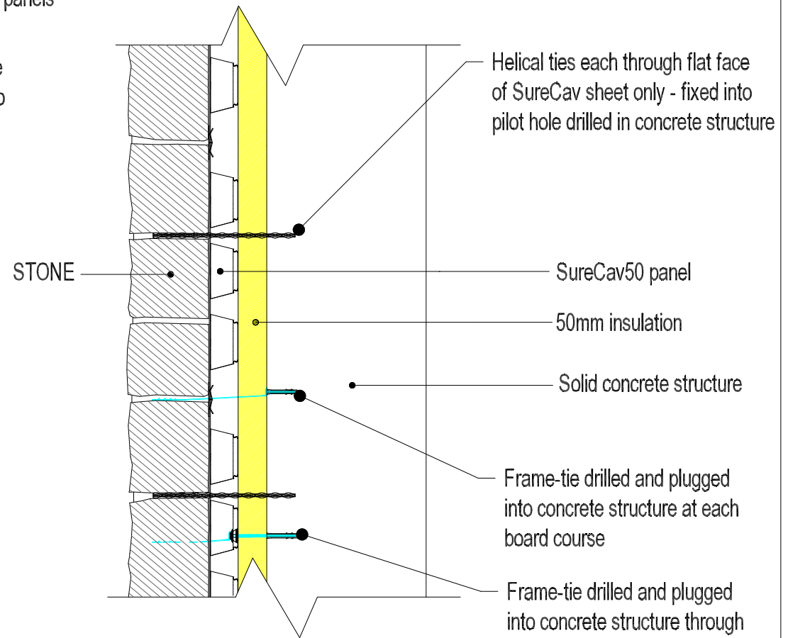
SURECAV50 WALL-TIE OPTION WITH SOLID CONCRETE STRUCTURE
